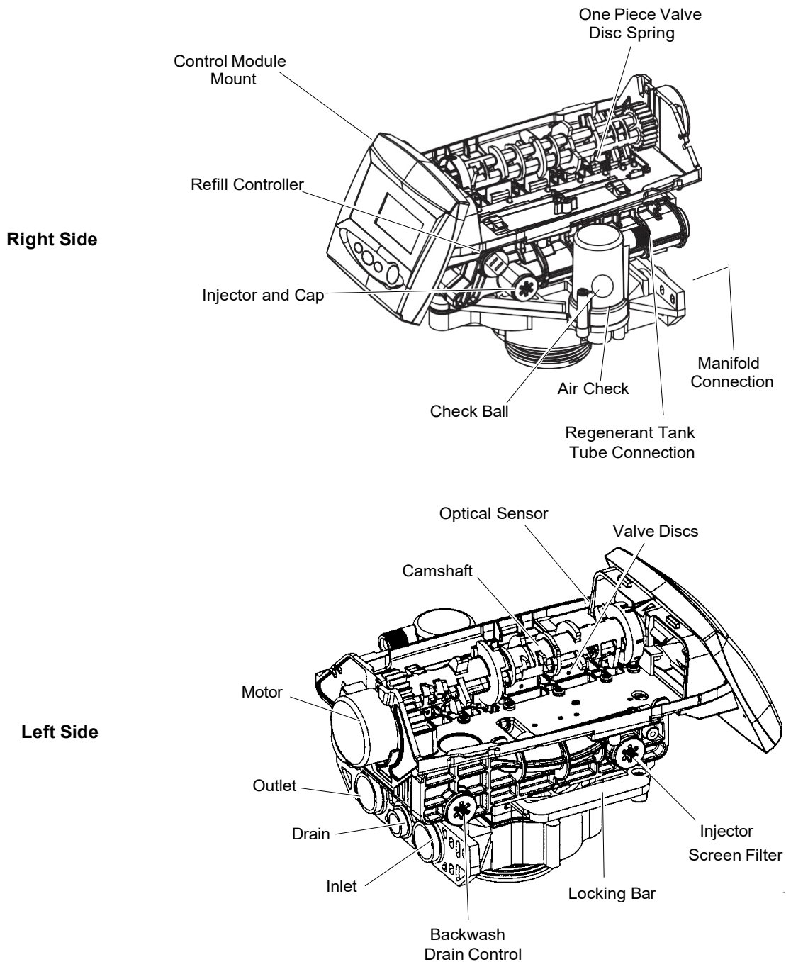
Figure 2 255 Valve Identification
